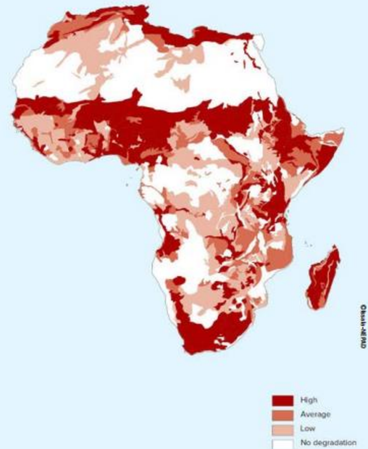
Soil Degradation
